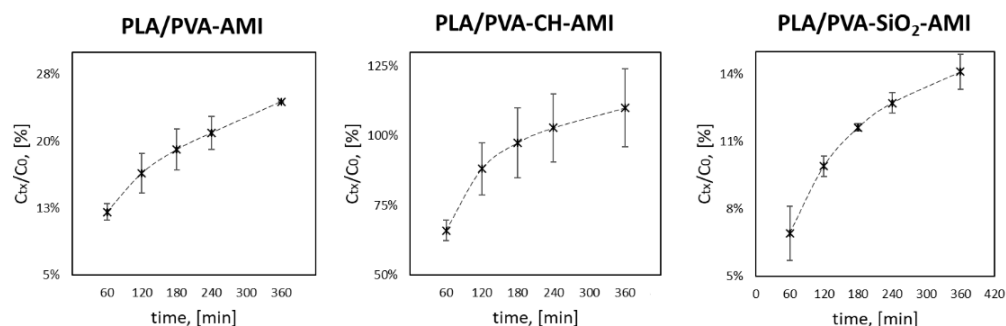
Figure 7. Simulation of AMI release according to OECD guidelines ( C_{tx} —amount of AMI released after time t ; C_0 —total amount of AMI in the material tested, n = 3 ).
