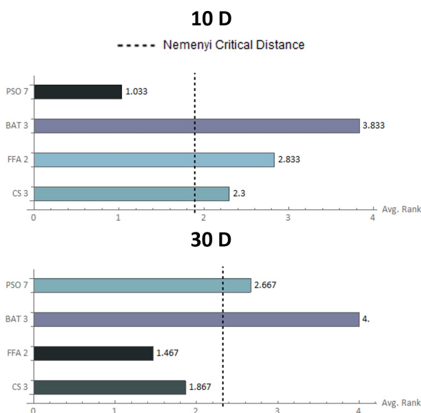
Figure 2: Example A: Friedman rank tests of the compared algorithms with parameter suited for 10 D.
