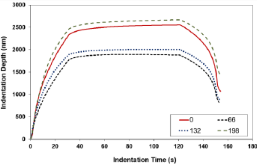
Figure 6: Indentation characteristic of tested PA 6
