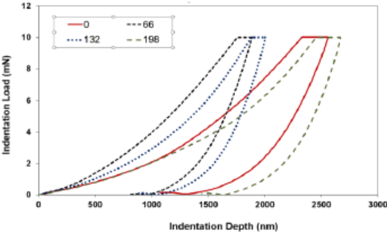
Figure 5: Indentation characteristic of tested PA 6
