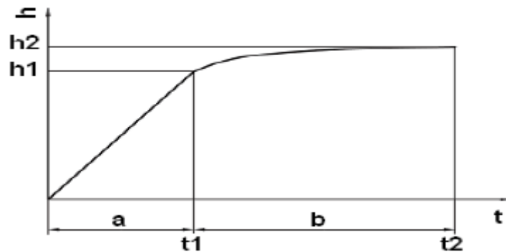
Figure 3: Expression of indentation creep, a - Application of the test force, b - Test force kept constant from t_1 to t_2 .
