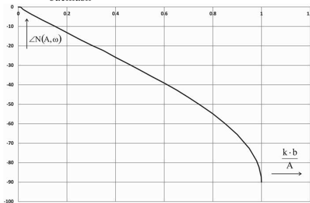
Fig.18. The describing function phase for the tooth backlash
