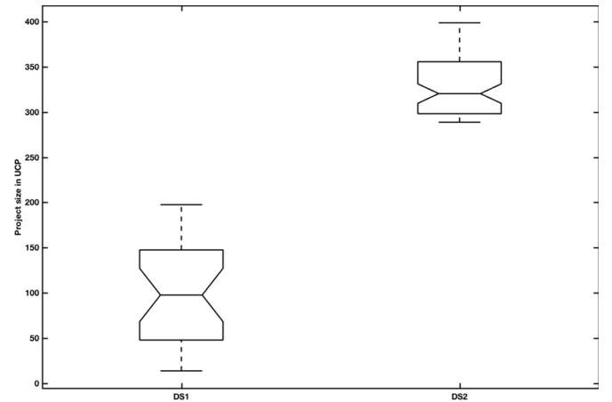
Fig. 3. Boxplots of project size, transformed into UCP.
