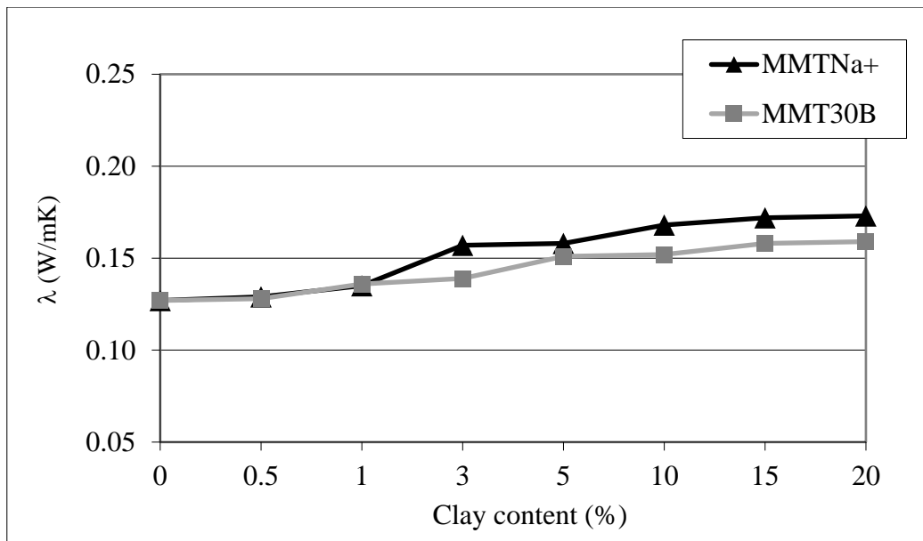
Fig.1. Thermal conductivity
