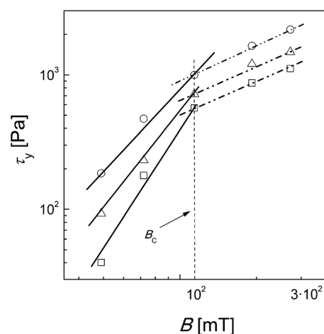
Fig. 10 Dependence of the yield stress, \tau_y , on the magnetic flux density, B , for particle silicone oil suspensions where (□) 80 wt% of bare CI, (△) 80 wt% of bare CI together with 1 wt% of sheet-like additive S3 and (○) 80 wt% of bare CI together with 5 wt% of sheet-like additive S3.
