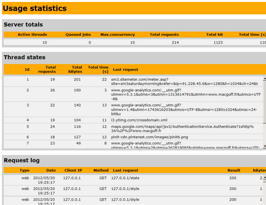
Fig. 2. Proxy Server GUI – statistic.
