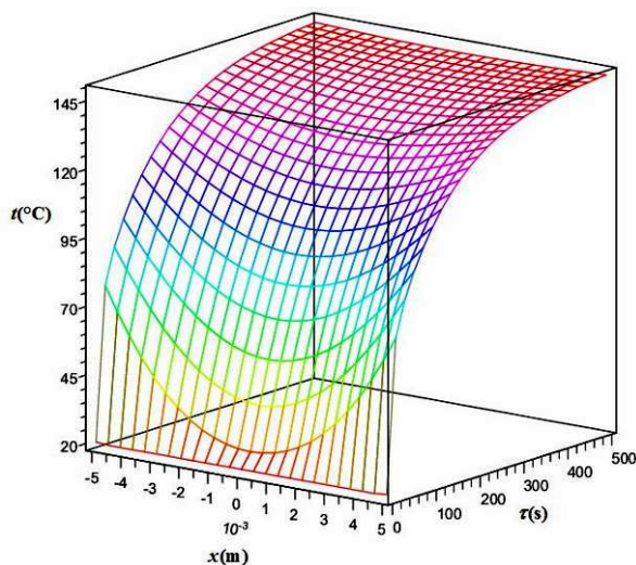
Fig. 3 Temperature field in a plate during symmetric heating. Parameters: t_p = 20 \text{ }^\circ\text{C} , t_o = 150 \text{ }^\circ\text{C} , a = 9,6 \cdot 10^{-7} \text{ m}^2\text{s}^{-1}
