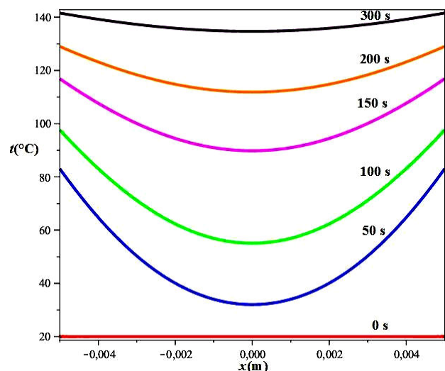
Fig. 3 Temperature field in a plate during symmetric heating. Parameters: t_p = 20 \text{ }^\circ\text{C} , t_o = 150 \text{ }^\circ\text{C} , a = 9,6 \cdot 10^{-7} \text{ m}^2\text{s}^{-1}
