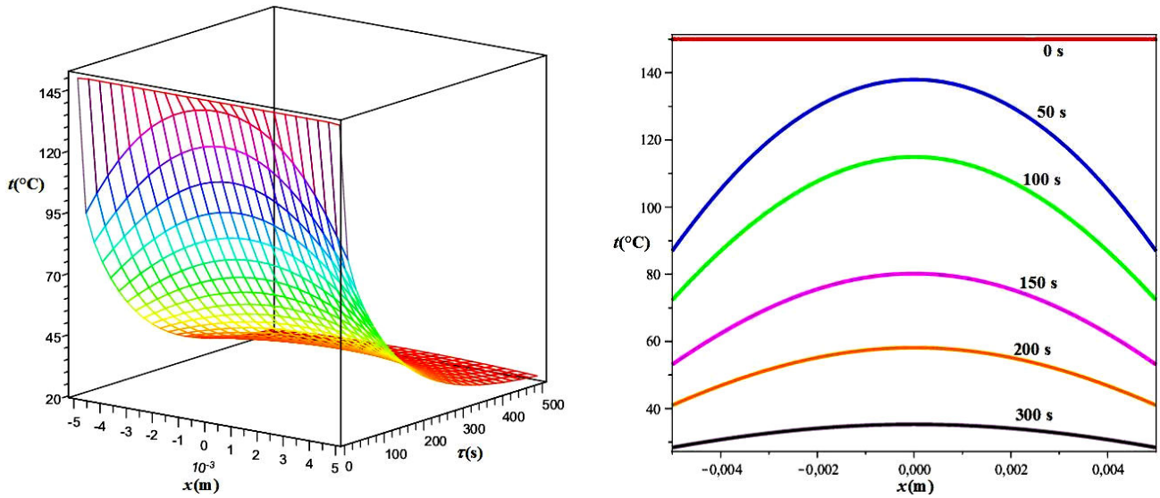
Fig. 4 Temperature field in a plate during symmetric cooling. Parameters: t_p = 150^\circ\text{C} , t_o = 20^\circ\text{C} , a = 9,6 \cdot 10^{-7} \text{ m}^2\text{s}^{-1}
