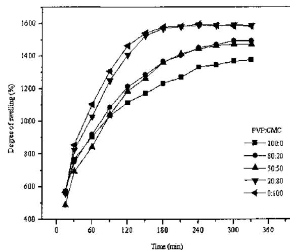
Figure 3 Swelling behavior of hydrogels.
