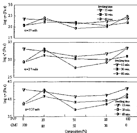
Figure 7 Effect of composition and swelling time on complex viscosity( r|^{*} ) at different angular frequencies ( \omega ) for the samples prepared with different swelling time.
