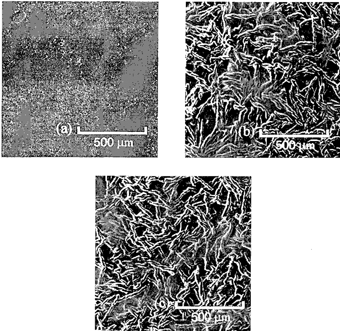
Figure 1 SEM micrographs of (a) PVP/CMC = 100 : 0, (b) PVP/CMC = 0 : 100, and (c) PVP/CMC = 20 : 80 samples.
